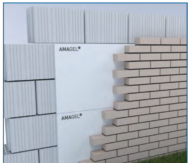
CAVITY WALLS
