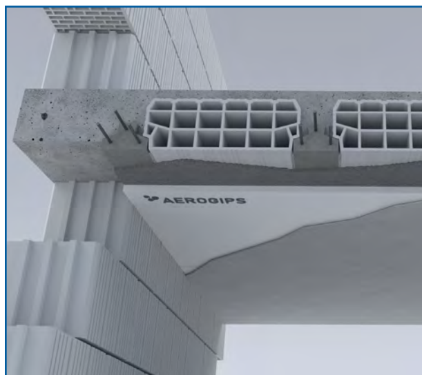
SOFFIT SLABS
