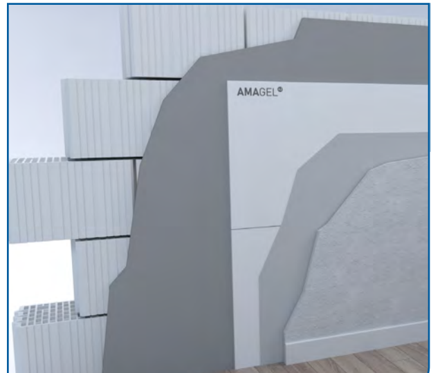
INTERNAL WALLS
